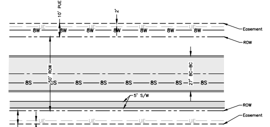
Typical Utility Layout
